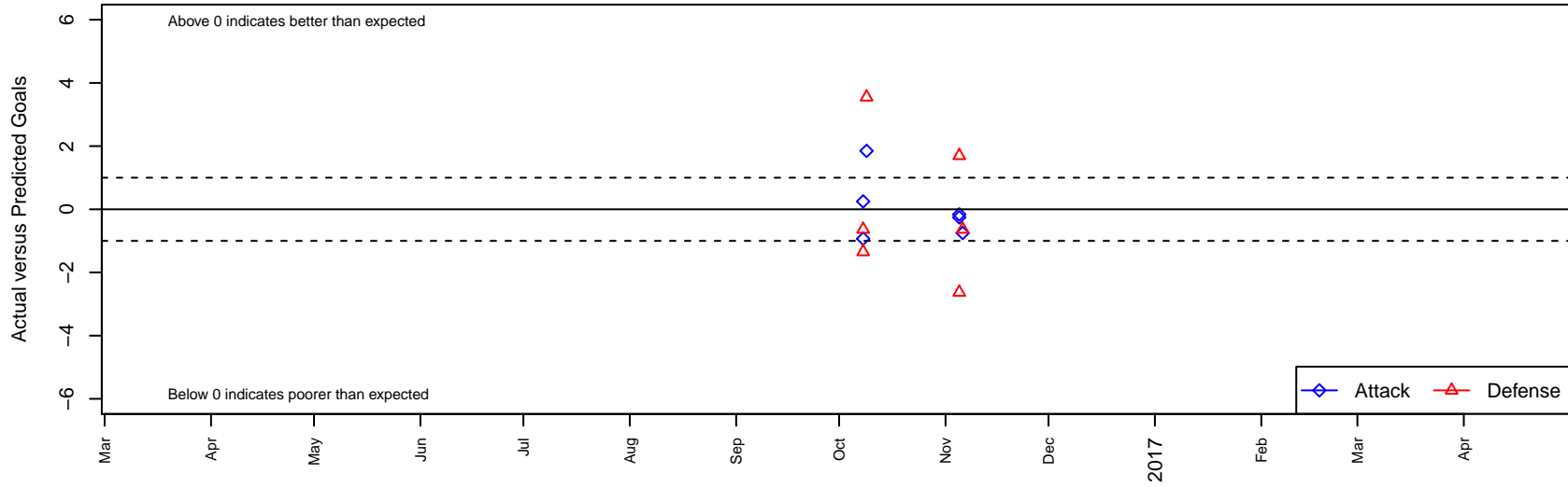
Jackson Hole United G05 Dots are actual minus expected GF (blue circles) and GA (red triangles). Blue line is smoothed change in attack strength. Red is smoothed change in defense strength.
